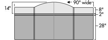
4 & 6 Panel Double-Arch
